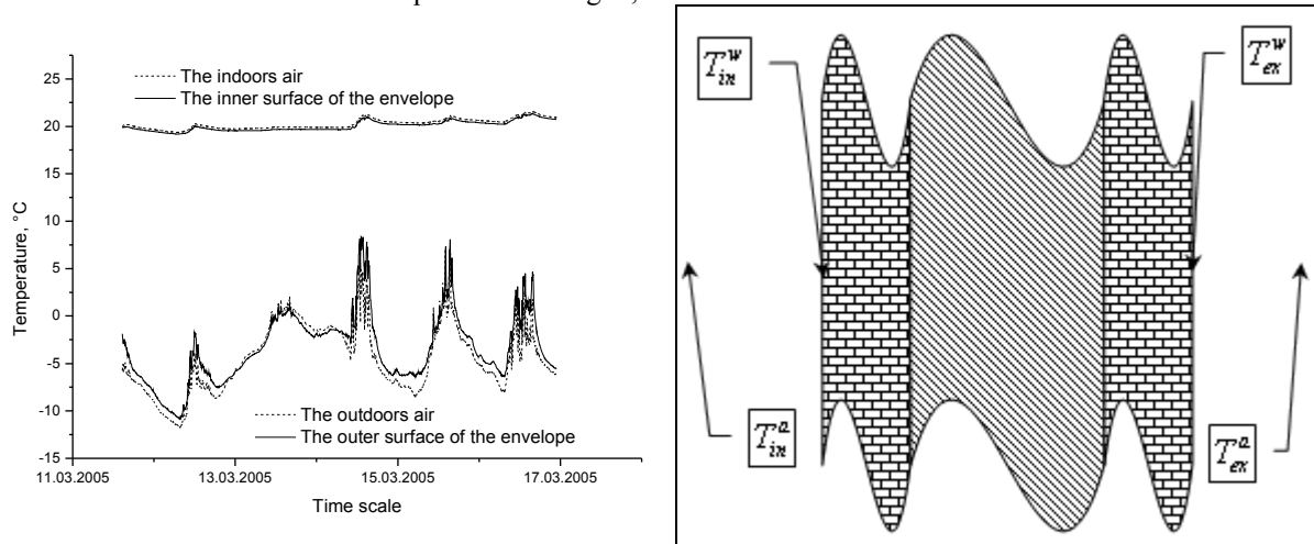
Fig. 2. Typical temperature time series of the reference zone (left). Sensor position at the reference zone (right).
